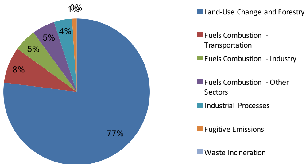
Figure 15: Sectoral Distribution of the CO 2 -emissions of Brazil in 2005 (own figure based on data from MCT Brazil, 2010, p. 138)
