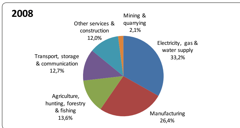
Figure 37: Greenhouse Gas Emissions of the EU by Sector in 2008 [CO 2 -equivalent] (own figure, based on Eurostat, 2012)
