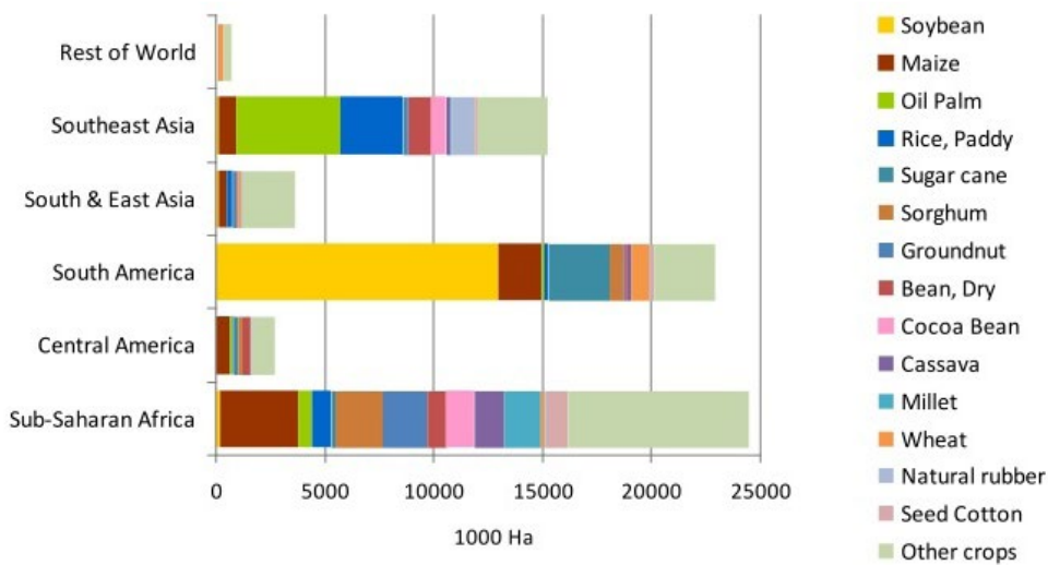
Figure 11: Share of Crops in Deforestation: Soybean as the Most Important Crop Causing Deforestation in South America, Period: 1990 – 2008 (Ermolieva et al. , 2012, p.83, reproduced with permission from the International Institute for Applied Systems Analysis (IIASA))
